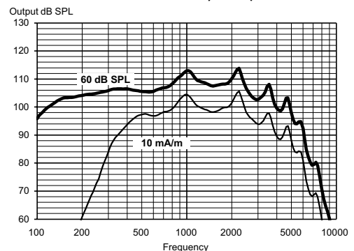
OUTPUT - 2CC COUPLER ANSI S3.22 (2009)
